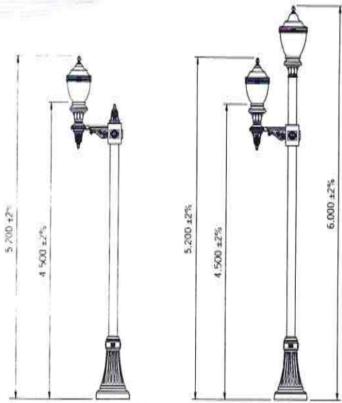
PDR 843B Q-11 / 45LL G
